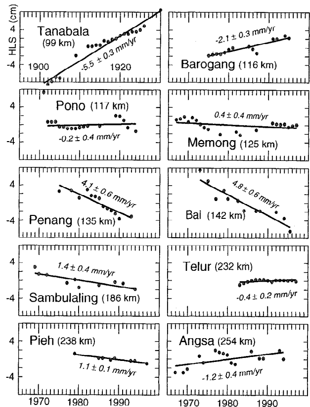
Figure 3. Representative coral HLS histories (in cm) with least-square linear fits. The HLS reference level is arbitrary. Note that the Tanabala record spans an earlier interval. The number in parentheses cites distance from the trench.
