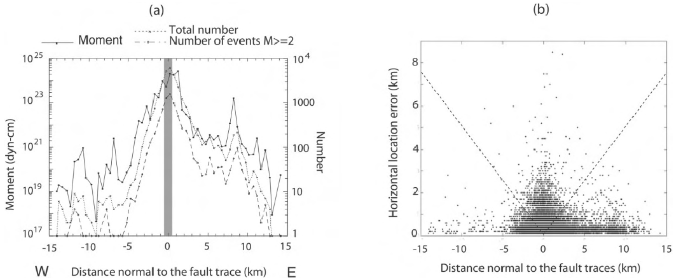
Figure 6. (a) Distributions of Landers aftershocks and (b) their horizontal location errors as a function of distance normal to the mainshock faults as shown in Figure 5, using relocated data set by Hauksson (2000). Only about 40% of the aftershocks occurred within 0.5 km of the mainshock faults. If we shift all aftershocks toward the nearest mainshock faults by the amounts of their 2\sigma location uncertainties, 44% of aftershocks might have occurred on the faults (those between the two diagonal dashed lines in Fig. 6b).
