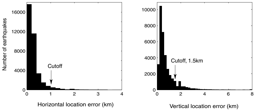
Figure 2. Histograms of horizontal and vertical location errors of relocated 1992 Landers aftershocks from 28 June 1992 to 22 May 1998. Relocations by Hauksson (2000). We excluded aftershocks with location errors greater than 1 km in the horizontal and 1.5 km in the vertical to avoid the use of ill-located aftershocks in our analysis.
