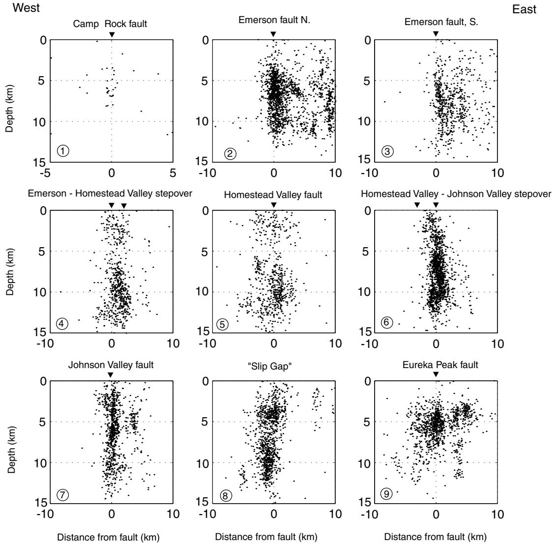
Figure 4. Cross-sectional views of aftershock locations ( M_L \geq 2 ) for the nine sections shown in Figure 1. The inverted solid triangles denote traces of the principal mainshock ruptures. Aftershock clouds suggest nearly vertically dipping mainshock fault planes, because the clouds do not spread out just to one side of the principal ruptures.
