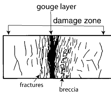
Figure 8. Schematic model of the gouge layer-damage zone morphology of a natural fault. It consists of a narrow gouge layer bounded by a broad damaged zone of subsidiary faults. The fracture density in the damage zone generally decreases with distance away from the center (modified from Wallace and Morris, 1986).
