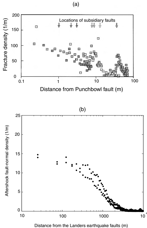
Figure 9. Density distributions of (a) mesoscopic fractures of the Punchbowl fault (Chester and Logan, 1986) and (b) Landers aftershocks as a function of distance normal to the principal fault plane. The fault-normal density of Landers aftershocks is summed over the entire length of the mainshock surface ruptures. The aftershock density at the center of the fault is 15 aftershocks per meter of distance perpendicular to the fault.
