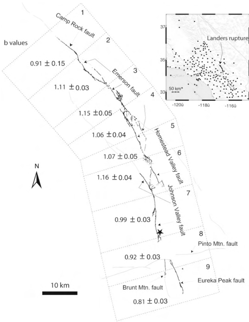
Figure 1. Map of the surficial ruptures of the 1992 Landers earthquake. The rupture is divided into nine sections for an examination of aftershock locations in cross-sectional views. Aftershock b -values in these sections range from about 0.8 to 1.2. Sections in which the rupture is simple have lower b -values, and sections of complex rupture have higher b -values. The inset figure shows the distribution of seismic stations during the period of the Landers aftershock sequence used in this article.
