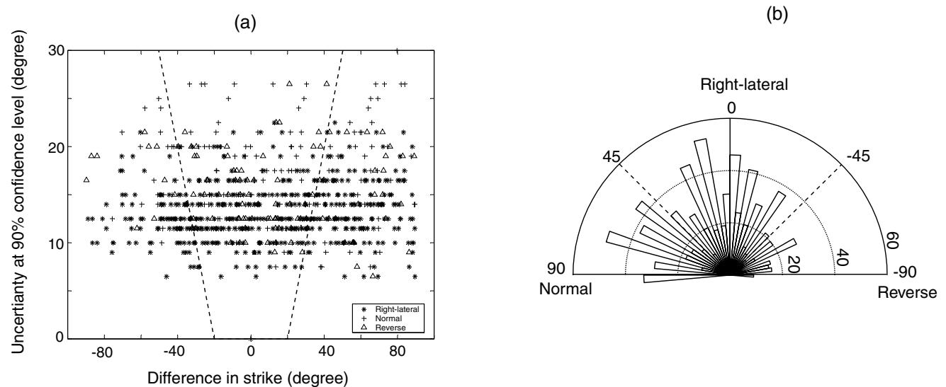
Figure 7. (a) The difference in strike of aftershock focal plane with that of the local mainshock fault is plotted against the uncertainty in strike of aftershock focal plane. We include only the 751 aftershocks that fall within 0.5 km of the mainshock rupture and have reliable first-motion solutions; 42% of these aftershocks are within 20^\circ of the local strike at the 90% confidence level (those between the two dashed lines). (b) The histogram of the sense of motion (rake) on the chosen plane. Right-lateral refers to those that have a larger horizontal component than vertical.
