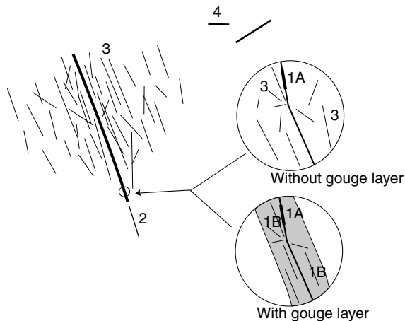
Figure 10. Schematic diagram illustrates the classification of aftershocks with respect to their locations relative to mainshock fault planes. See text for the definition for each class of aftershocks.
