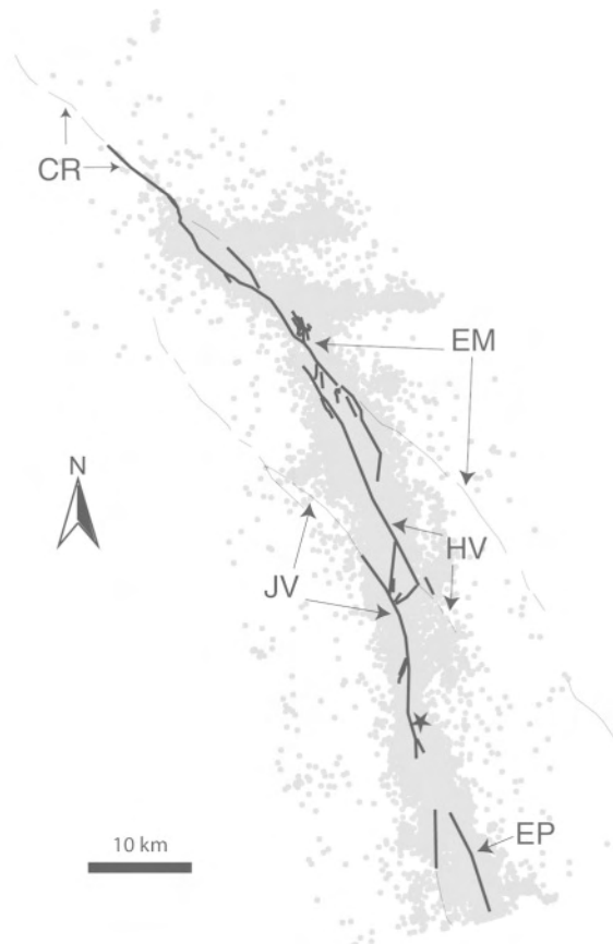
Figure 5. Map view of the surface traces of the mainshock fault planes and aftershock locations. Simplified surface ruptures, shown as thick lines, represent the fault planes that failed during the mainshock; fault planes beyond the ends of the mainshock ruptures are shown as thin lines. Abbreviations of the faults are the same as in Figure 3.
