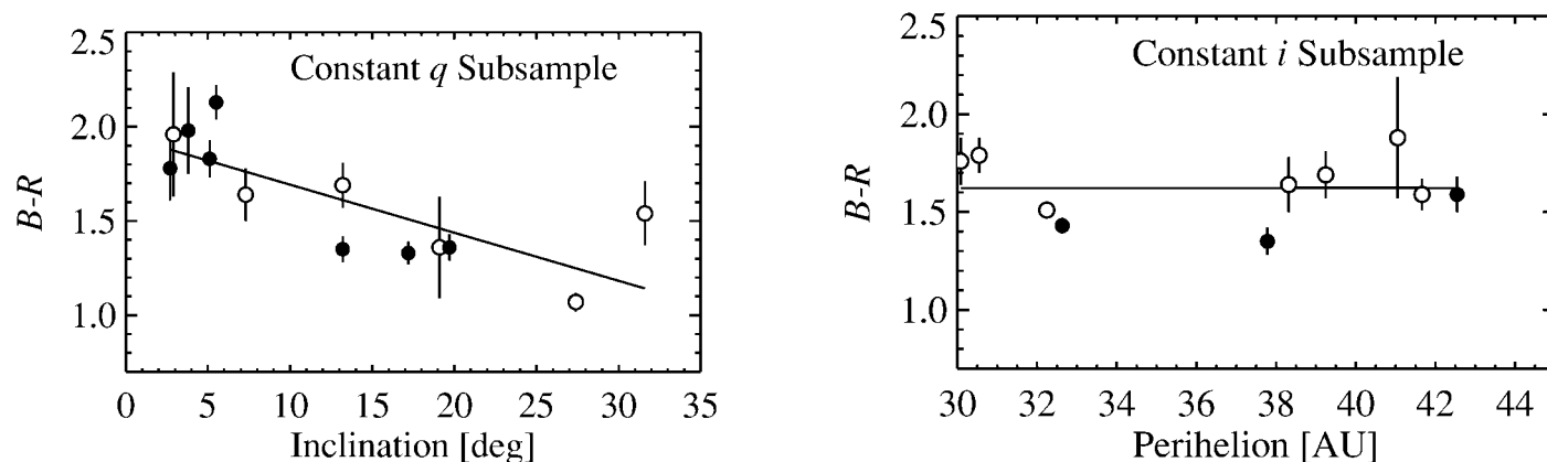
FIG. 3.—Color vs. inclination for the constant q subsample ( left ) and color vs. perihelion for the constant i subsample ( right ). The left panel corresponds to 2.8\sigma , and the right panel is not significant, as estimated by the Spearman rank correlation method. The constant perihelion subsample ( left ) indicates that the inclination/color correlation is not due to observational bias. In contrast, the constant i subsample lacks any trend, indicating that the observed perihelion/color correlation is most likely due to sampling bias induced by the perihelion/inclination correlation.
