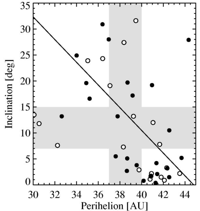
FIG. 2.—Inclination vs. perihelion for the classical KBOs and scattered KBOs in our sample (filled circles) and all published data (no Plutinos; open circles). For illustrative purposes, a linear least-squares fit has been plotted for points with perihelion greater than 34 AU (solid line). The gray bars represent the constant q (vertical bar) and constant i (horizontal bar) subsamples detailed in Fig. 3.
