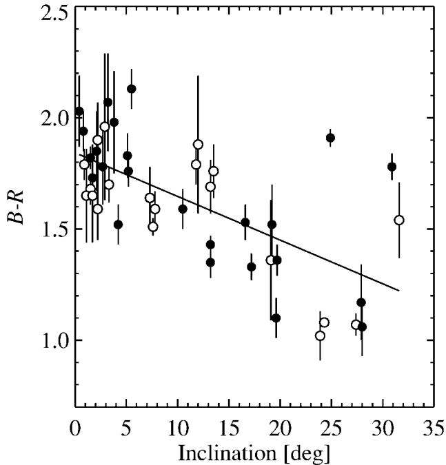
FIG. 1.— B-R color vs. inclination for the classical KBOs and scattered KBOs in our sample (filled circles) and all published data (no Plutinos; open circles). A linear least-squares fit has also been plotted for illustrative purposes (solid line; slope = -0.0196 \pm 0.003 \text{ mag deg}^{-1} , intercept = 1.84 \pm 0.5 \text{ mag} ). The trend corresponds to 3.1 \sigma (our data points) and 4.1 \sigma (all data points) significance, as estimated by the Spearman rank correlation method.
