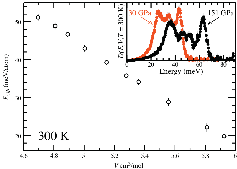
Fig. 1. The volume-dependent vibrational free energy per ^{57}\text{Fe} atom ( F_{\text{vib}} ) at 300 K. Inset shows the measured total phonon DOS of \epsilon -Fe at 30 GPa (red) and 151 GPa (black) at 300 K. (For interpretation of the references to color in this figure legend, the reader is referred to the web version of this article.)
