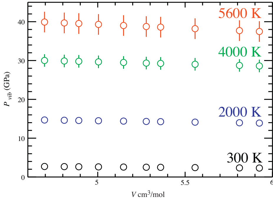
Fig. 2. The volume- and temperature-dependent vibrational thermal pressure ( P_{vib} ) of \epsilon -Fe. P_{vib}(T > 300 \text{ K}) account for anharmonic effects, and errors calculated from best-fit parameters are smaller than the symbol if not visible.
