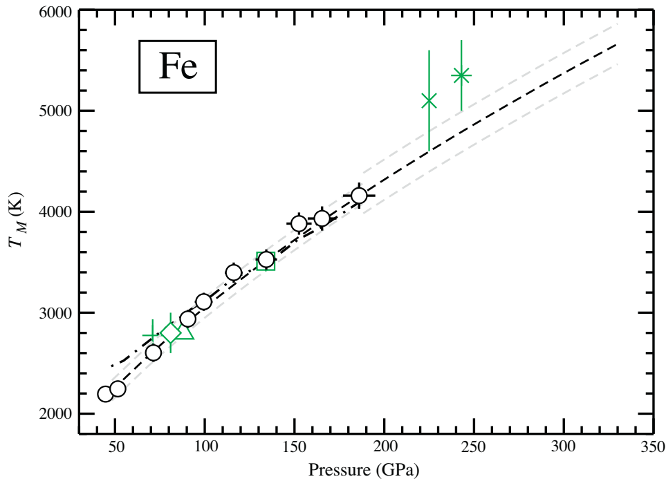
Fig. 3. The high-pressure melting behavior of \epsilon -Fe. Black circles show melting points that account for thermal pressure and anharmonic effects. The black dashed line gives the fit and extrapolation of our melting points with Eq. (11), and the gray dashed lines show uncertainties of \pm 100 K over our experimental compression range, and \pm 200 K beyond our compression range. The black dash-dotted line shows our harmonic melting temperatures, which account for thermal pressure. The green x , + , and * show results from shock-compression melting experiments by Nguyen and Holmes (2004), Ahrens et al. (2002), and Brown and McQueen (1986), respectively; the green triangle, square, and diamond show results from static-compression XRD experiments by Komabayashi and Fei (2010), Ma et al. (2004), and Shen et al. (1998), respectively, where the final two have been corrected to account for thermal pressure following Eq. (10). (For interpretation of the references to color in this figure legend, the reader is referred to the web version of this article.)
