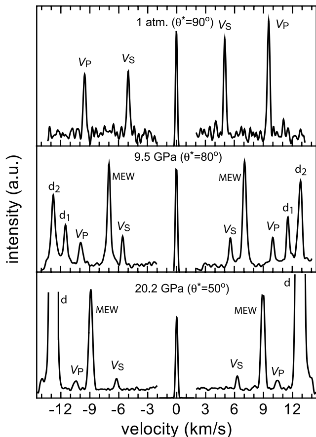
Figure 1. Representative Brillouin spectra at different pressures (1 atmosphere, 9.5 GPa, and 20.2 GPa) and at different scattering geometries ( \theta^* ) of Fp06 in approximately the [011] phonon direction within the (100) crystallographic plane. The 1 atm. spectrum was collected outside the DAC. The compressional ( V_P ) and shear ( V_S ) wave velocities of Fp06 are labeled, as well as the methanol-ethanol-water compressional wave velocity (MEW) and the diamond shear velocities ( d_1 , d_2 ). In all spectra, the peak corresponding to the reference energy (velocity = 0 km/s) has been scaled down. The intensity axes for each pressure are not equal; in the lower spectrum, the diamond peak intensities are larger than the scale shown. Direct conversion of the measured data (in units of GHz) to the horizontal scale shown here (velocity, in units of km/s) requires knowledge of the momentum transfer (i.e., the scattering angle) and is done using equation (1) (see text).
