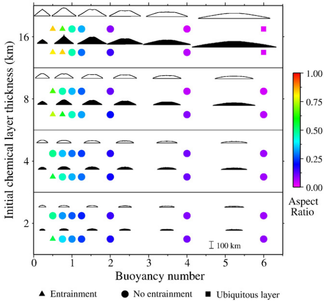
Fig. 5. Aspect ratio (relief/half-width) of the structures at steady-state. See Fig. 3 caption for legend.
