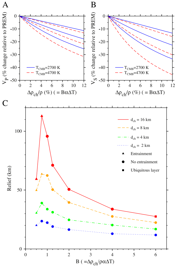
Fig. 7. (A and B). Voigt–Reuss–Hill (VRH) wavespeed determinations at two end-member CMB temperature estimates for the “PREM + Mw” mixing model. Voigt (upper), Reuss (lower), Hill (arithmetic average). See text for model details. (C) Relief of structures for the impermeable cases.
