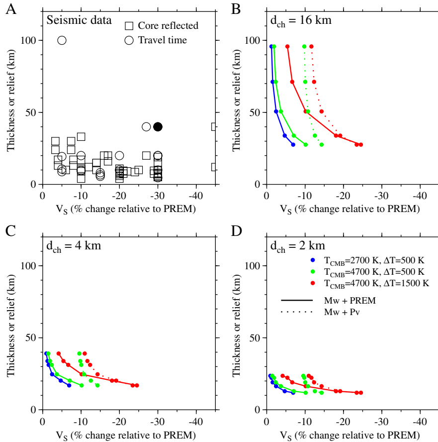
Fig. 9. (A) Seismically inferred ULVZ thicknesses and S-wave velocity reductions found globally. Following the nomenclature of Garnero and Thorne (2004): \square precursors to core reflected phases (Avants et al., 2006; Garnero and Vidale, 1999; Havens and Revenaugh, 2001; Hutko et al., 2009; Kohler et al., 1997; Reasoner and Revenaugh, 2000; Rost and Revenaugh, 2003; Rost et al., 2005, 2006, 2010a), \circ travel time and waveform anomalies (Garnero and Helmberger, 1995; Helmberger et al., 1998, 2000; Ni and Helmberger, 2001a; Rondenay and Fischer, 2003; Simmons and Grand, 2002; Thorne and Garnero, 2004; Wen and Helmberger, 1998b; Zhang et al., 2009). Filled symbols denote 2-D studies. (B, C, and D) Models using the Hill bound, for various d_{ch} , temperature at the CMB ( T_{CMB} ), and temperature drop ( \Delta T ). Solid lines are the “Mw + PREM” model and dotted lines are the “Mw + Pv” model.
