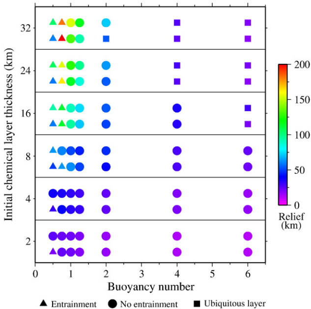
Fig. 2. Relief of the structures at steady-state. For each initial chemical layer thickness, data points corresponding to the impermeable cases are located above the points for the permeable cases. 'Ubiquitous layer' refers to cases where the chemical layer occupies the full lateral extent of the domain.
