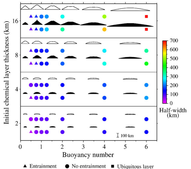
Fig. 4. Half-width of the structures at steady-state. See Fig. 3 caption for legend.
