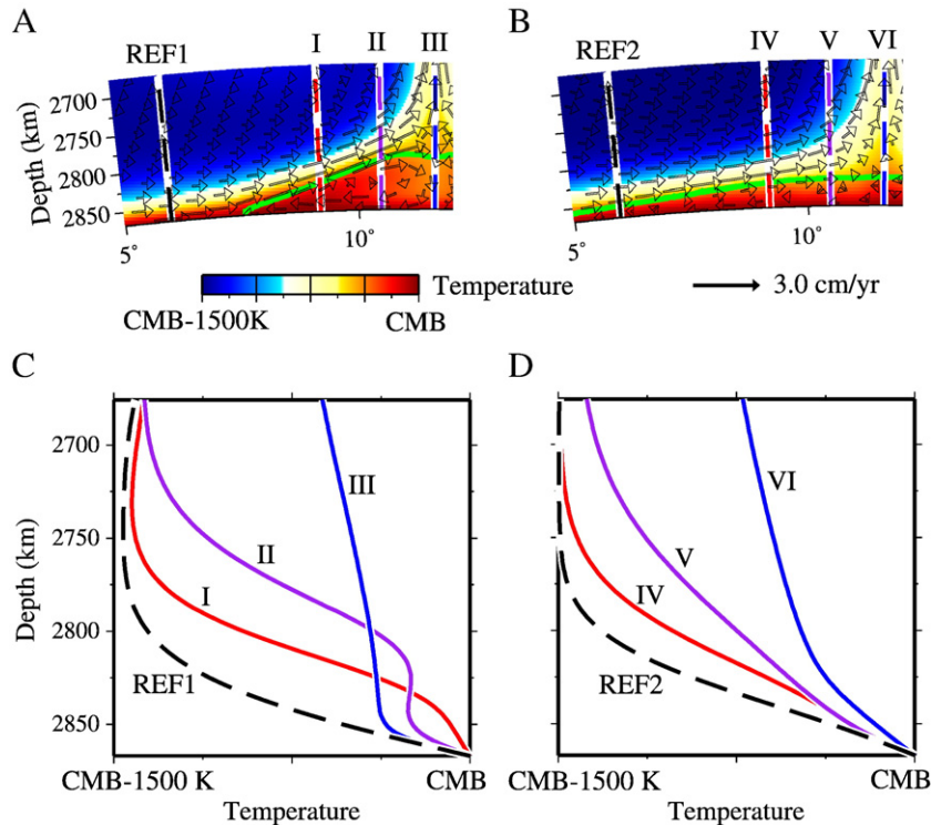
Fig. 6. Steady-state behavior of a thin (Mg,Fe)O-containing layer. (A) Counter-circulation driven by viscous coupling ( B=1.25 , d_{ch}=16 km, impermeable domain). The ULVZ component is contained within the area outlined in green and the CMB. (C) Temperature profiles: reference REF1, upwelling I, center II, and downwelling III. (B) Sluggish convection ( B=6 , d_{ch}=16 km permeable domain). (D) Temperature profiles (REF2, IV, V, VI) are at the same locations as in (C).
