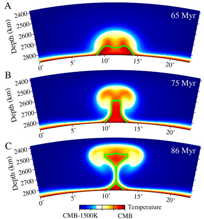
Fig. 1. Representative behavior during the transient period for a model with a low chemical density anomaly and hence entrainment ( B=0.5 , d_{ch}=16 km, impermeable domain). The ULVZ component is contained within the area outlined in green and the CMB. (For interpretation of the references to color in this figure legend, the reader is referred to the web version of this article.)
