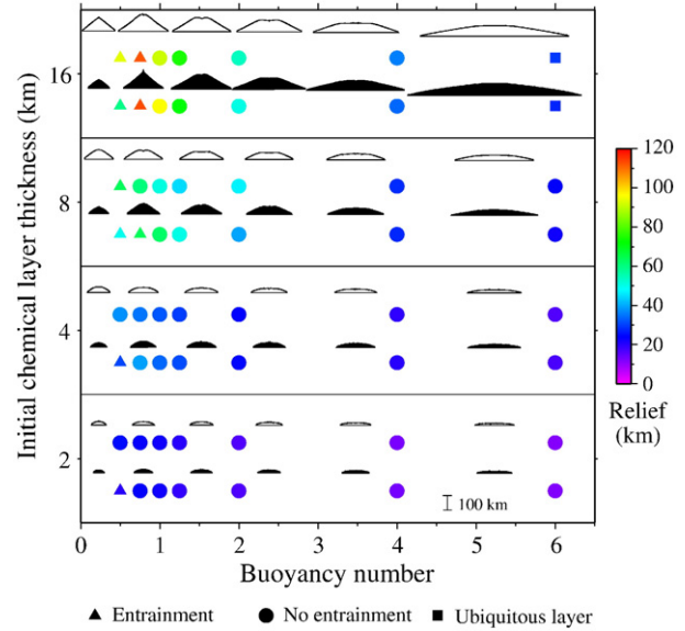
Fig. 3. Relief of the structures at steady-state. The morphologies for B = 0.5 to B = 4 , plotted to scale, are shown in successive order from left to right above their corresponding data points. For B = 6 the morphologies are omitted because of space consideration but are comparable to B = 4 . Permeable cases: black outline, impermeable cases: black fill. Note color scale is different in Fig. 2. (For interpretation of the references to color in this figure legend, the reader is referred to the web version of this article.)
