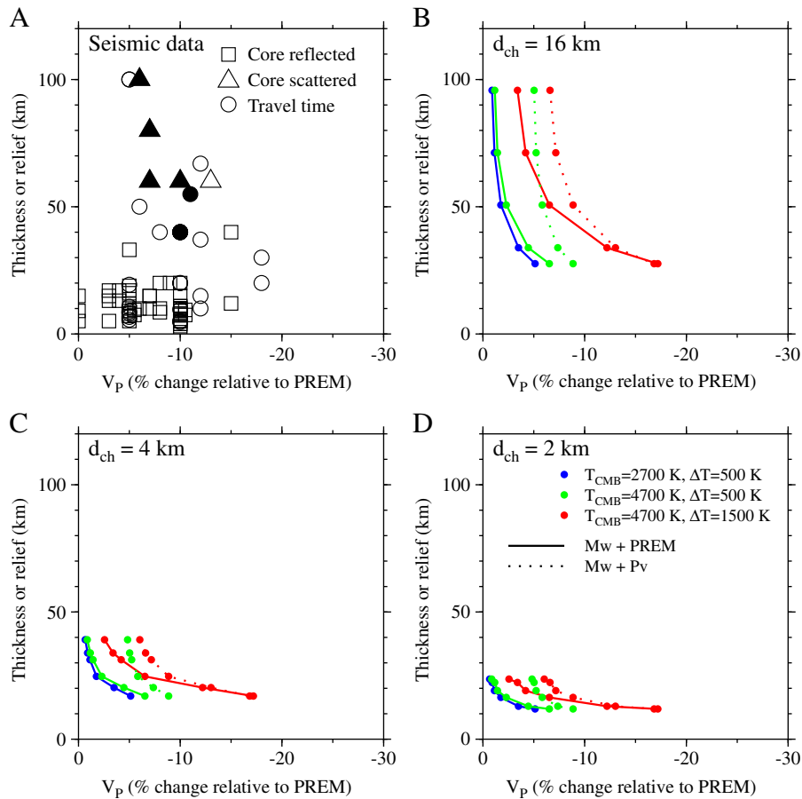
Fig. 8. (A) Summary of seismically inferred ULVZ thicknesses and P-wave velocity reductions found globally. Following the nomenclature of Garnero and Thorne (2004): □ precursors to core reflected phases (Garnero and Vidale, 1999; Havens and Revenaugh, 2001; Hutko et al., 2009; Kohler et al., 1997; Mori and Helmberger, 1995; Reasoner and Revenaugh, 2000; Rost and Revenaugh, 2003; Rost et al., 2005, 2006, 2010a), △ scattered core phases (Ni and Helmberger, 2001b; Niu and Wen, 2001; Vidale and Hedlin, 1998; Wen and Helmberger, 1998a), ○ travel time and waveform anomalies (Garnero and Helmberger, 1995; Garnero and Helmberger, 1996; Garnero et al., 1993; Helmberger et al., 1996, 1998, 2000; Luo et al., 2001; Ni and Helmberger, 2001a; Rondenay and Fischer, 2003; Simmons and Grand, 2002; Thorne and Garnero, 2004; Wen, 2001; Wen and Helmberger, 1998b). Filled symbols denote 2-D studies. (B, C, and D) Models using the Hill bound, for various d_{ch} , temperature at the CMB ( T_{CMB} ), and temperature drop ( \Delta T ). Solid lines are the “Mw + PREM” model and dotted lines are the “Mw + Pv” model.
