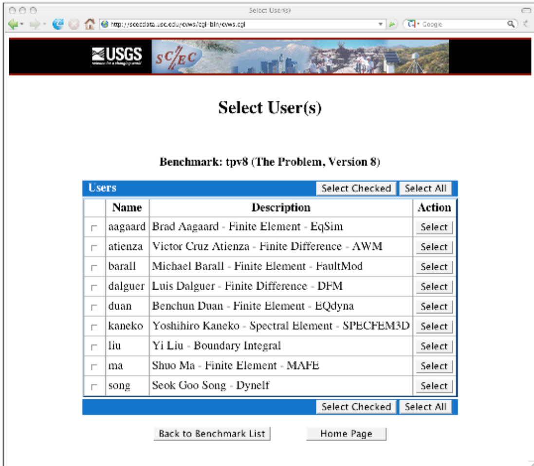
Figure 4. One of the code comparison webpages. This public webpage lists the modelers and fully operational codes that performed the TPV8 benchmark. The specifications for this benchmark are outlined in Table 1, and provided in detail on the webpage http://scecddata.usc.edu/cvws/benchmark_descriptions.html
