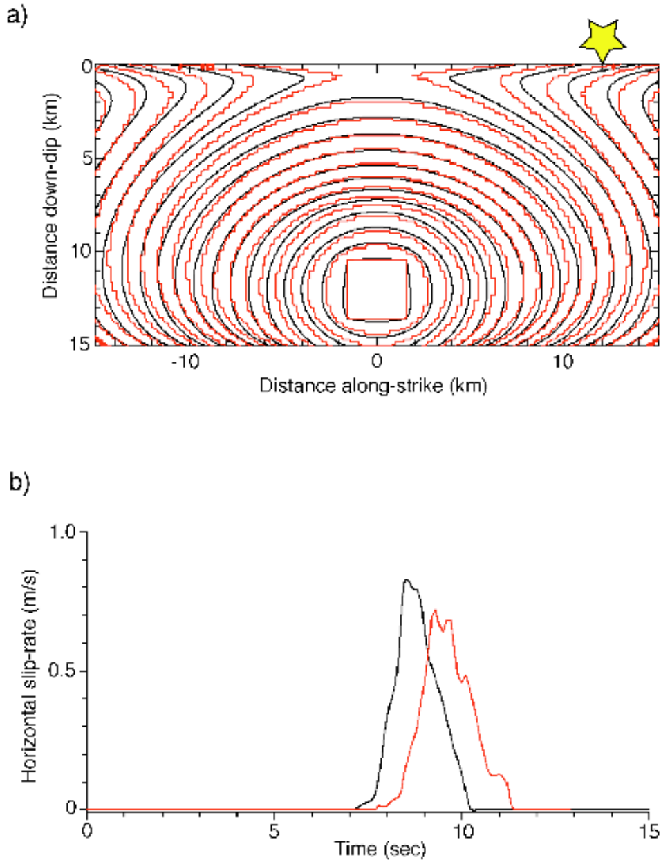
Figure 5. Webpage showing results for two spontaneous rupture codes that ran the TPV8 benchmark. One code is still in the developmental stage and so does not appear in the public section of the website, the other code is in the operational stage and does appear in the public section of the website. Comparisons show a) the rupture-front contour plots, that indicate where, at 0.5-second contoured intervals, the earthquake rupture first slipped the fault at \geq 1 mm/s, and b) the horizontal slip-rates in m/s at an on-fault station that is 12-km along strike from the epicenter. The station location is indicated by the star in part a). Both the rupture-front contour plots and the synthetic seismograms qualitatively indicate a relatively poor match between these two codes.
