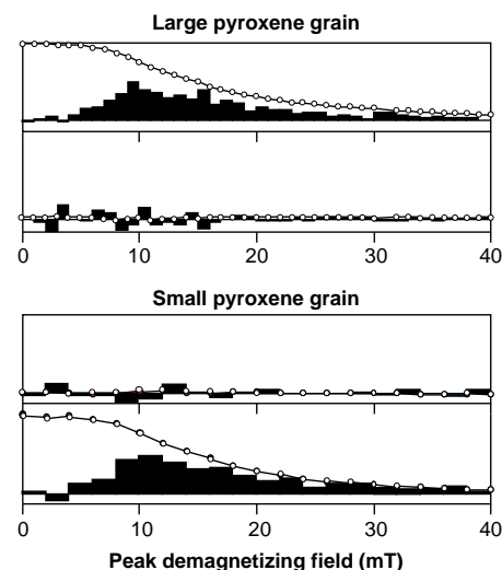
Fig. 4. Comparison of the coercivity spectra for components A1 and B, from the large and small pyroxene grains, respectively. This is a test for the presence of the large pyroxene A1 direction in the smaller grain, and vice versa. Demagnetization data were transformed from the orthogonal X, Y, Z Cartesian system of the magnetometer to a right-canted system using the normal direction vectors parallel to A1, B, and their cross-product (A1 × B). Normalized coefficients of components A1 and B are plotted as a function of the peak demagnetization field for both samples, and the histograms show the relative fraction removed between successive demagnetization steps. The vertical axis shows the scalar intensity of each component, normalized to the maximum moment for each sample. This deconvolution indicates that no consistent component of the large pyroxene grain's A1 direction is present within the smaller grain, and, similarly, no consistent component of direction (B) from the small pyroxene grain is present in the large grain. The coercivity spectra of components A1 and B overlap completely above the 5-mT level.
