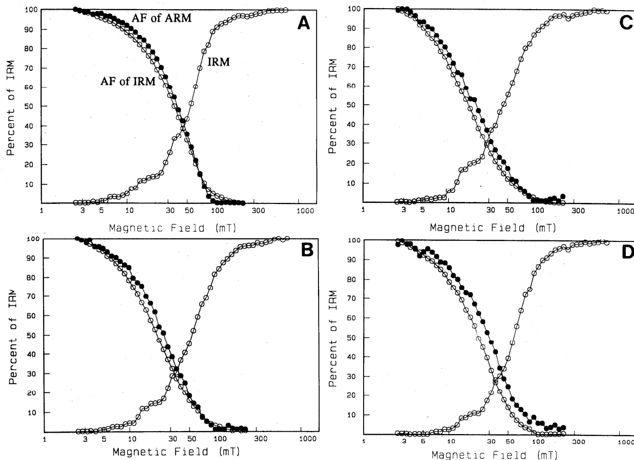
Fig. 6. Coercivity spectra for limestones and dolomite: (a) modern submarine cemented sediments, Joulters Cay Bahamas; (b) calcitic limestone, core UNDA, 28.8 m; (c) fabric preserving dolomite from core GB-1, 74.3 m; and (d) fabric destructive dolomite from San Salvador, 96 m.
