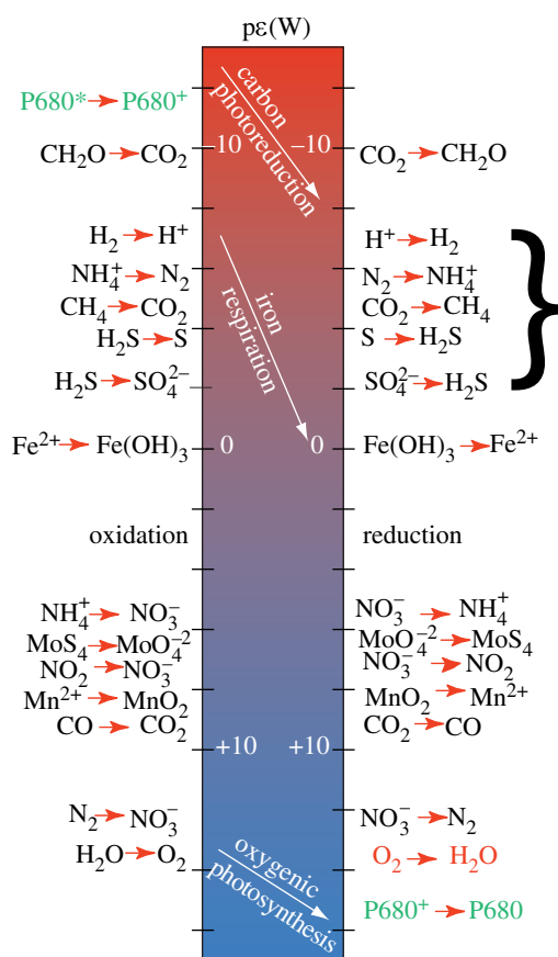
Figure 1. Electron activity ( pe ) of typical redox couples in water at pH 7 and 25°C (adapted from Gaidos et al. 1999). Half-reactions on the left couple spontaneously with those below them on the right, and most pairs are suitable for driving biological metabolism. The primary donor of PSII (P680) has the largest redox potential change known for any organic molecule, and in its oxidative (rest) state, it is capable of oxidizing water, producing oxygen. The thick bracket signifies the range of gases emitted from volcanic eruptions. Subaerial eruptions tend to be more oxidizing than subaqueous eruptions, so the shift in eruptive style towards subaerial volcanism noted by Kump & Barley (2007) would have helped the eventual oxidation of the atmosphere, even though all volcanic gases are on the reducing side of the ferrous/ferric couple. Note that the term ‘oxidizing’ appears to have quite separate meanings in the geological and biological sciences. Redox couples near the quartz–fayalite–magnetite buffer in rocks are considered oxidizing by the Earth scientists, but are actually on the reducing side of the diagram and clearly faraway from the NO_3^- and O_2 couples considered oxidizing by biologists.
