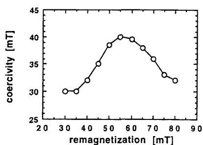
FIG. 2. Effect of the pulse remagnetization technique on the median coercivity of cultures of A. magnetotacticum . As discussed in the text, north-seeking cultures of A. magnetotacticum were exposed at increasing magnetic pulses, reisolated, and grown and had their coercivity distribution measured.
