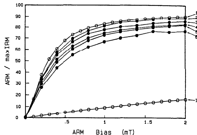
FIG. 3. ARM acquisition of different enrichments of A. magnetotacticum after the pulse remagnetization treatment. Open circles represent the characteristic pattern displayed by noninteracting single-domain particles obtained from A. magnetotacticum curve 1 and fully interacting single-domain particles from chiton teeth (7) (curve 7). The ARM curve of the wild-type strain of A. magnetotacticum overlapped with the uppermost curve (curve 1). Curves 2 to 6 represent the ARMs observed in samples obtained after 40, 50, 60, 70 and 80 mT of pulse remagnetization, respectively. ARM values along the ordinate were also normalized to the maximum IRM value for each sample.
