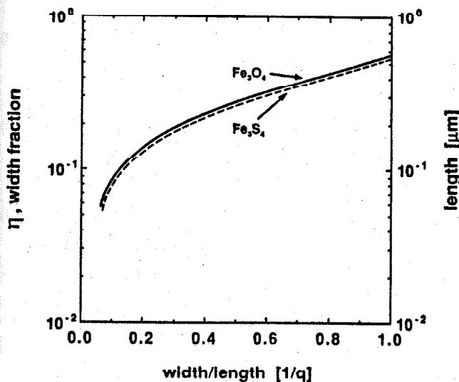
Fig. 6. Width ratio of the 180^{\circ} boundary wall ( \eta = wall width/grain width) and length of different grains of greigite ( \text{Fe}_3\text{S}_4 ) and magnetite ( \text{Fe}_3\text{O}_4 ) as a function of the shape (width/length).
