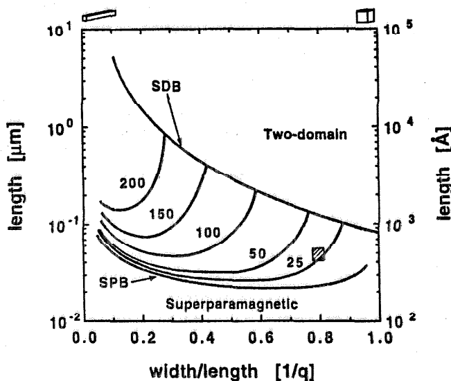
Fig. 4. Single-domain stability diagram for magnetite prisms. SD-SPM boundary (SPB) and SD-2D boundary (SDB) were calculated using J_s = 480 \text{ emu/cm}^3 , \tau = 100 \text{ s} , T = 290^\circ\text{K} , \sigma_0 = 0.8 \text{ erg/cm}^2 , and \delta_0 = 1.5 \cdot 10^{-5} \text{ cm} . Coercivities ( H_b ) are expressed in milliteslas. The square represents the location of an average single domain crystal of magnetite assuming an axial ratio ( 1/q ) equal to 0.8, length a = 0.05 \text{ }\mu\text{m} [Mann et al., 1987b], and bulk coercivity H_b = 30 \text{ mT} [Mann et al., 1987a]. Assuming values of \sigma_0 and \delta_0 as mentioned above, for a cubic grain, d_0 is 0.082 \text{ }\mu\text{m} .
