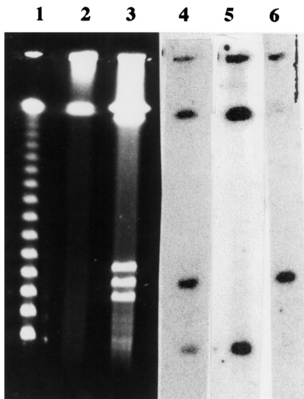
Fig. 3. Localization of genes to an extra-chromosomal structure. Plugs of MS-1 DNA were digested with the restriction enzyme SwaI and subjected to PFGE, using a run time of 20 h and a switch time of 13–54 s. The gel, minus the lambda ladder, was subsequently blotted onto a nylon membrane (see Section 2.5), which was probed sequentially with \alpha^{32}\text{P} -dCTP-labelled insert DNA. The radioactivity was stripped off between probes. Lane 1, lambda 50 kb ladder; lane 2, undigested DNA; lane 3, SwaI -digested DNA; lanes 4–6, SwaI -digested DNA shown in lane 3, probed with partial sequences of the 16S rRNA gene, the bra and por genes, and bfr genes 1 and 2, respectively.
