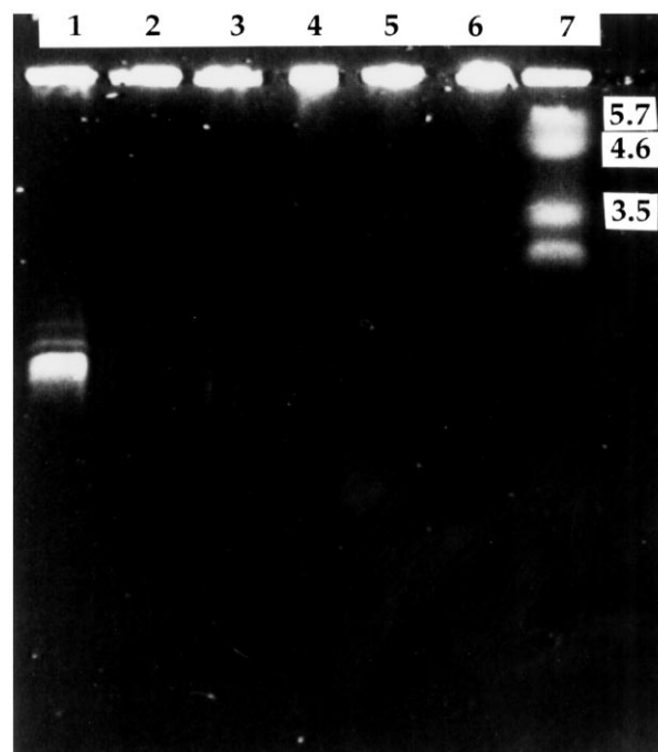
Fig. 2. Pulsed-field gels analysis of undigested MS-1 genomic DNA. One percent agarose gels were loaded with plugs of undigested, genomic MS-1 DNA and run in 1 × TAE buffer at 2 v/cm 2 for 72 h with a switch time of 2100 s. Lane 1, Sc chromosomes; lane 2, Ec DNA; lanes 3–5, MS-1 DNA; lane 6, Ad DNA; lane 7, Sp chromosomes, with the molecular weights (mb) indicated.
