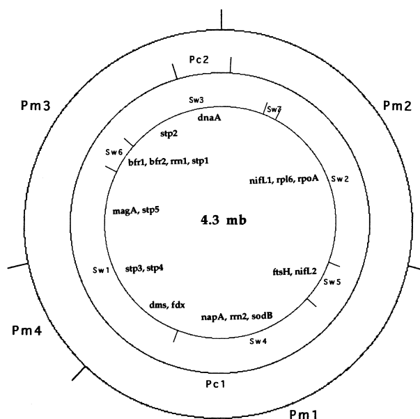
Fig. 4. Restriction and genetic maps of the MS-1 genome. Using the data in Tables 1 and 2, a restriction map produced by digestion of MS-1 DNA with the restriction enzyme PmeI is presented as 4.3 mb circle. The most probable arrangements of restriction fragments produced with enzymes PacI and SwaI are displayed as concentric circles within the PmeI map. The locations of some of the genes listed in Table 2 are indicated.
