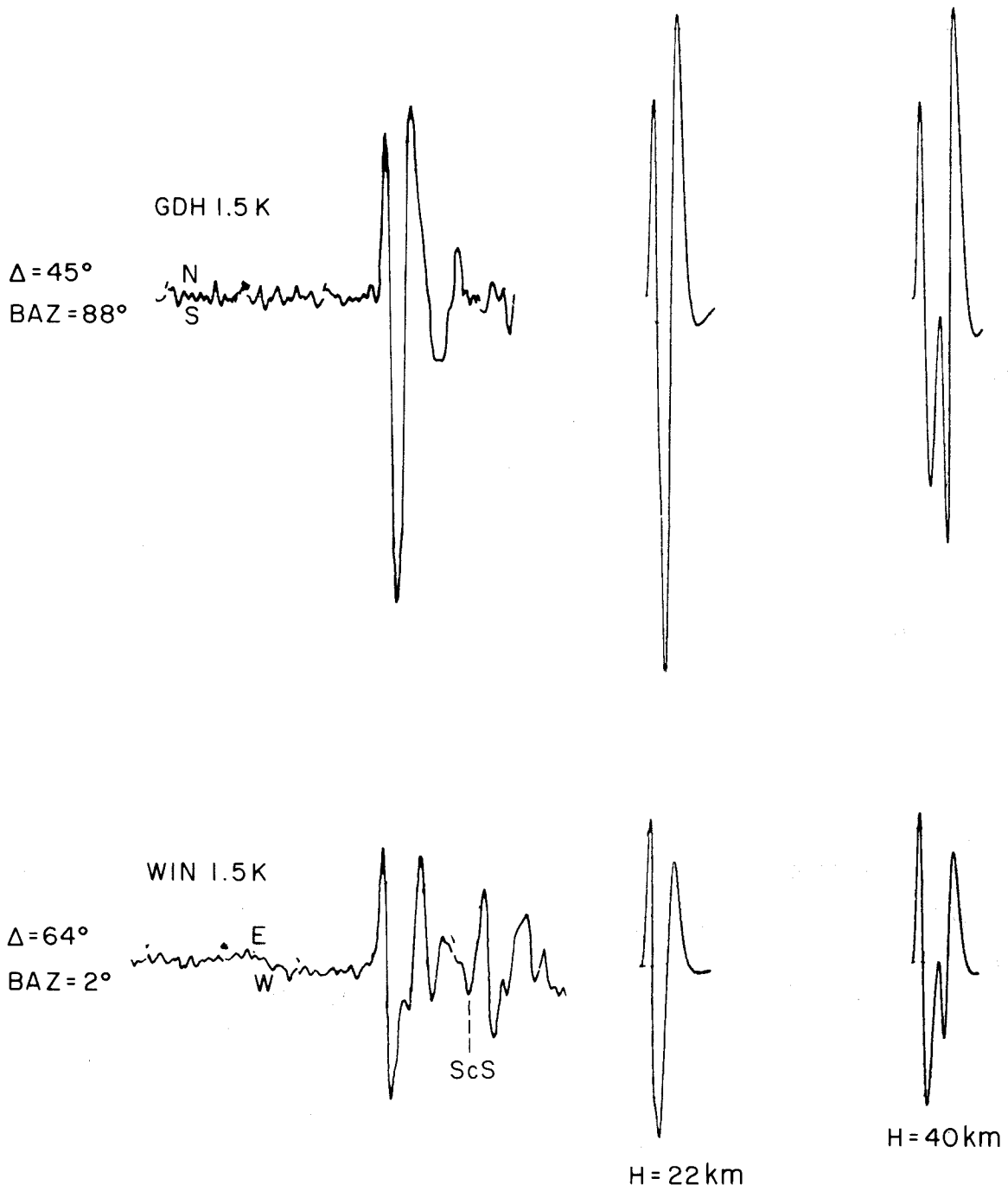
Fig. 7. Observed and theoretical S waves from a point-source model located at the depth indicated. All theoretical calculations assumed t^* = 4 and a moment of 1.0 \times 10^{19} Nm. The theory and data are plotted to the same scale. The derivative of the source time-function was approximated by a trapezoid with durations of 0.5 and 4.0 s for the shoulders and central section, respectively. A rake angle of 90^\circ (pure thrust) was used for plane A of figure 2.
