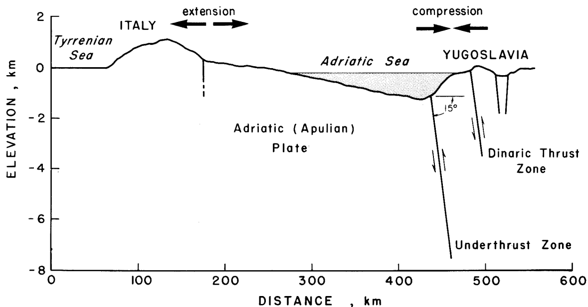
Fig. 3. Schematic southwest to northeast cross-section from Italy across the Adriatic Sea to Yugoslavia. The Montenegro earthquake probably occurred on the underthrust zone. The apparent steepness of the fault zones is an artifact of the vertical exaggeration ( \times 30 ) of the cross-section. Actual dip is probably 15° or less.
