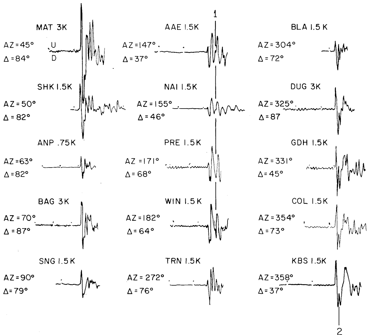
Fig. 5. Tracings of P waves arranged according to source-to-station azimuth (AZ). The magnification follows the station abbreviation. Phases 1 and 2 are discussed in the text.
