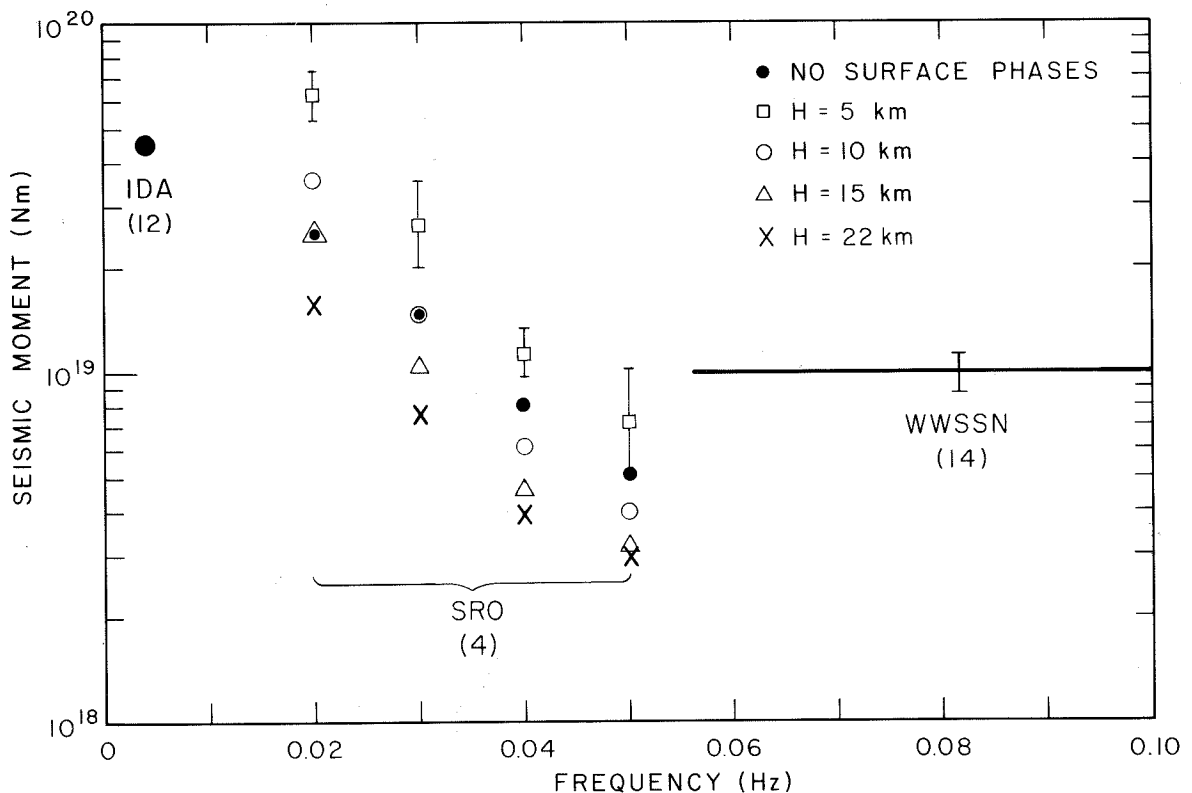
Fig. 4. Seismic-moment estimates. Number of records used in estimate in parentheses. Influence of source depth shown for SRO data. Bars are standard error of the means (shown for one source depth; errors for other points are similar). Logarithmic averages were used to compute means except for IDA estimate, based on an arithmetic mean. WWSSN estimates were based on first extreme of P- and S-wave arrivals with dominant periods about 10 and 20 s, respectively, and were only slightly affected by source depth. SRO estimates at each frequency were made assuming that the observed spectral level equalled the long-period spectral level. Corrections were made for instrument response, geometric spreading, radiation pattern, and attenuation ( t^*=4 ).
