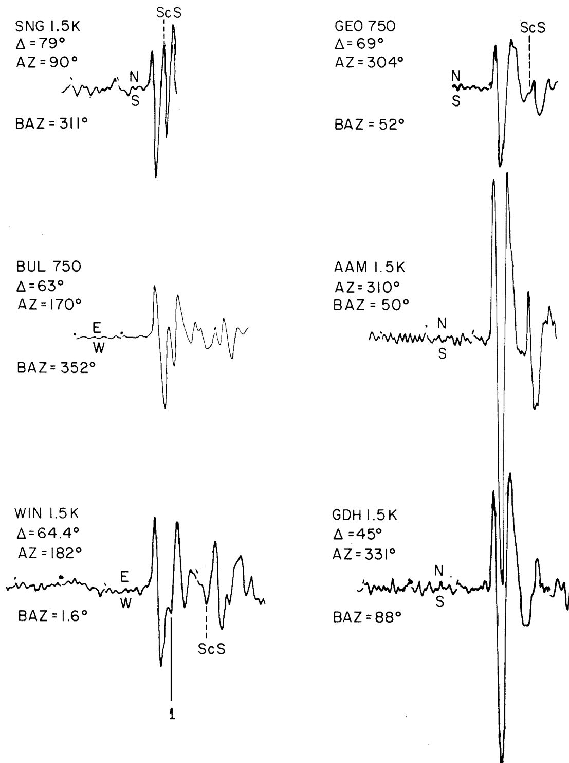
Fig. 6. Tracings of S waves arranged by source-to-station azimuth (AZ). The station-to-source (back) azimuth is given by BAZ. The S waves are predominately SH, being either naturally polarized into the transverse direction or having a transverse polarization, as seen by correlating both horizontal components (not shown).
