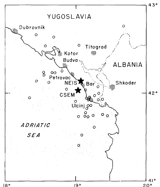
Fig. 1. Epicenters of main-shock (stars) and after-shocks (dots) of the Montenegro, Yugoslavia, earthquake of April 15, 1979. After-shock locations, taken from NEIS reports, for 1-day period after main-shock.
