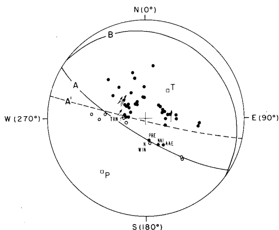
Fig. 2. P-wave focal mechanism solution (lower hemisphere, equal area projection): dots and circles are compressional and dilatational first motions, respectively; (N) a nodal first motion; (P, T) pressure and tension axes for the system of planes A, B; arrows are polarization vectors of S waves. Plane A' is mentioned in the Discussion section. Seismograms from named stations are shown in Fig. 5.
