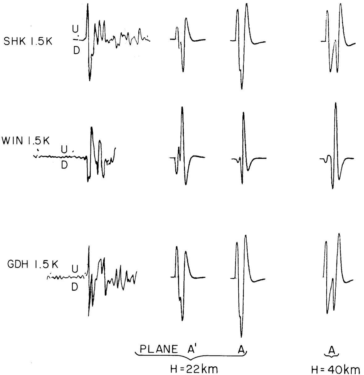
Fig. 8. Observed- and theoretical-P waves, as in Fig. 7 except a rake angle of 50^\circ (left-lateral, thrust) was used on plane A' and r^* = 1 .
