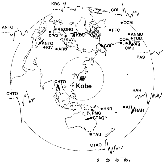
Fig. 3. IRIS broadband seismograph stations within teleseismic distance ( 30\text{--}100^\circ ). Waveforms show the initial portion of P-waves. The arrow indicates the initial polarity of the SH-waves.
