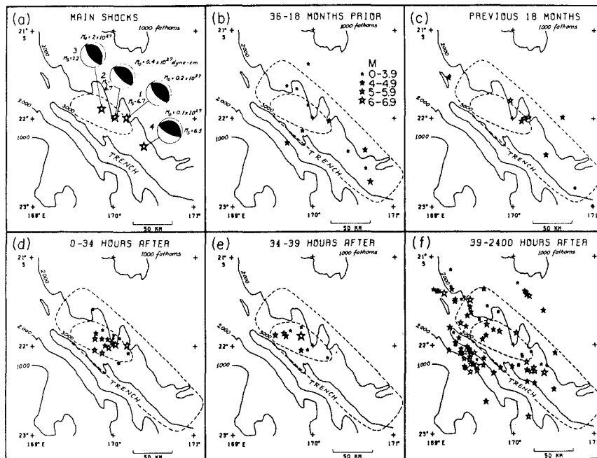
Fig. 2. Seismicity plots of the area covered by the black square in Figure 1. Stars indicate earthquakes; larger symbols indicate larger events. The solid lines contour the bathymetry (Mammerickx et al., 1974) in fathoms. Figure 2a shows the hypocenters, mechanisms, surface-wave magnitudes, and seismic moments for the four largest events in the sequence. Figures 2b and 2f show activity in 5 different time windows. The outer dotted line contains the later aftershock zone and was derived from Figure 2f. The inner dotted line contains the immediate aftershock zone and was drawn from Figure 2e.
