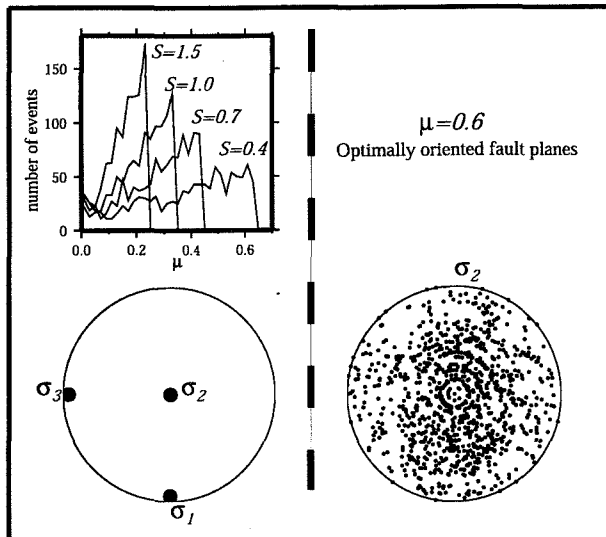
Figure 5. Summary figure showing the two end-member models. The left side shows the model in which a uniform stress is assumed. The lower-left figure shows the orientations of the principal stresses determined by inversion, and the upper-left figure shows the histograms of the events having friction \mu for the four models of S . The right side shows the model in which uniform friction \mu = 0.6 and optimally oriented fault planes are assumed. The lower-right figure shows the orientations of the intermediate stress axis.
