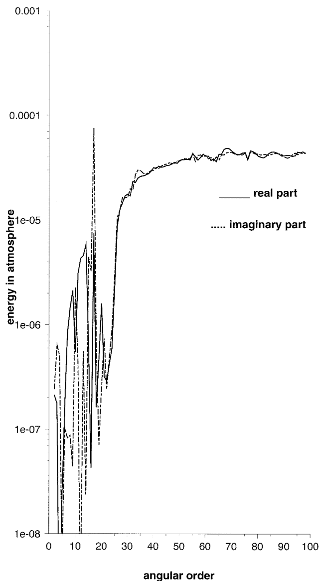
Figure 10. Same as Fig. 8 but for the second overtone of solid Earth modes.
