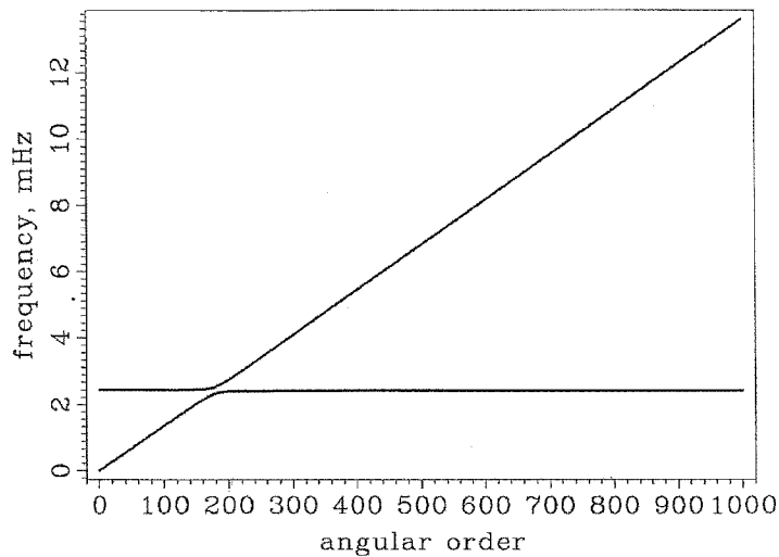
Figure B1. The two roots of eq. (B4) are shown with respect to the angular order \ell and the frequency. The domains for the trapped modes and for the propagating modes are indicated. These roots are calculated for the atmospheric model at 150 km, where the boundary condition is applied.
