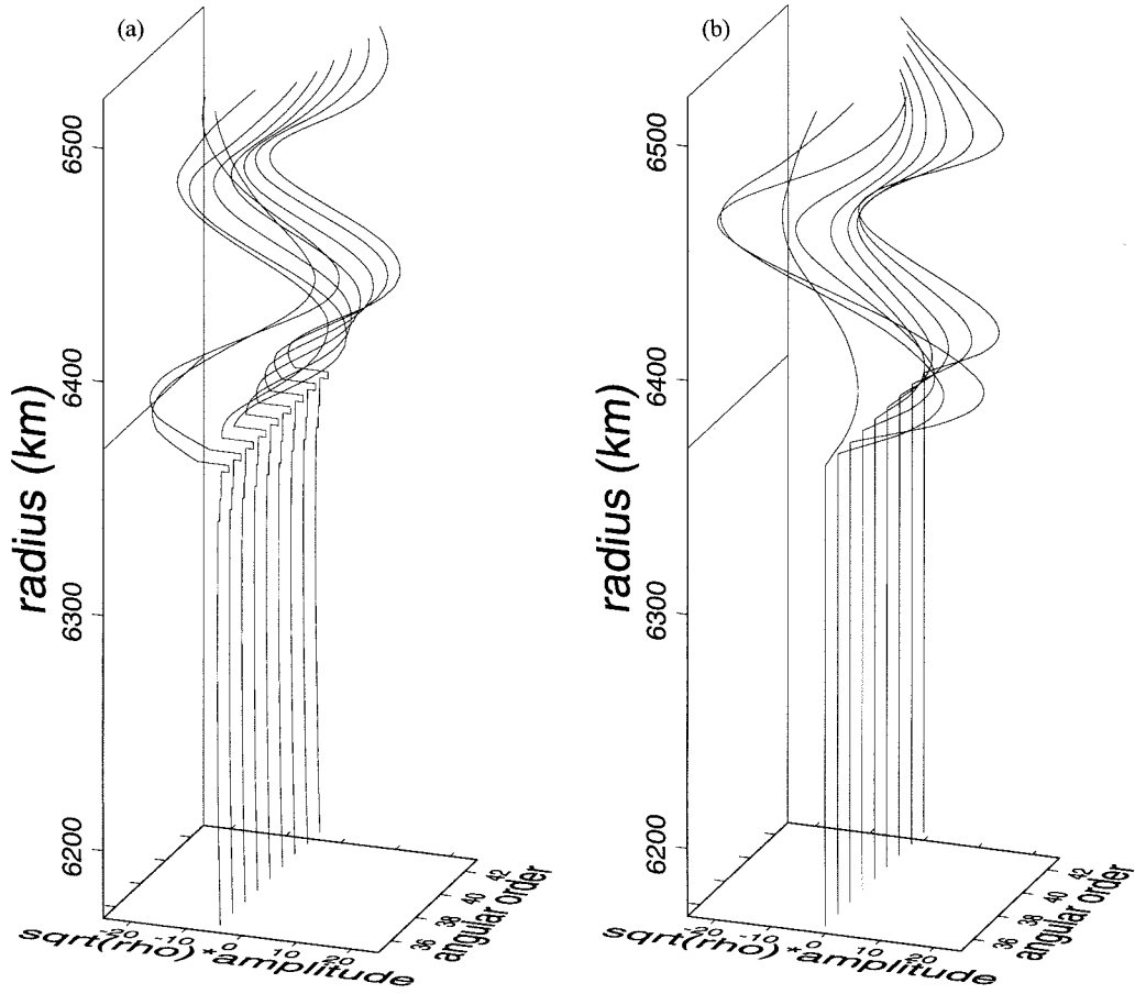
Figure 12. (a) Real part and (b) imaginary part of the solid Earth fundamental modes between \ell=35 and \ell=43 . These modes are around the second resonance at 4.40 mHz. Note that the imaginary part has comparable amplitude to the real part.
